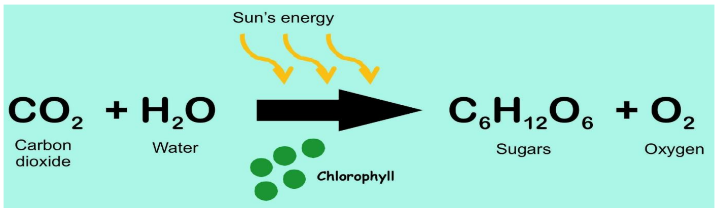
Fig.2. Overall Equation of Photosynthesis
